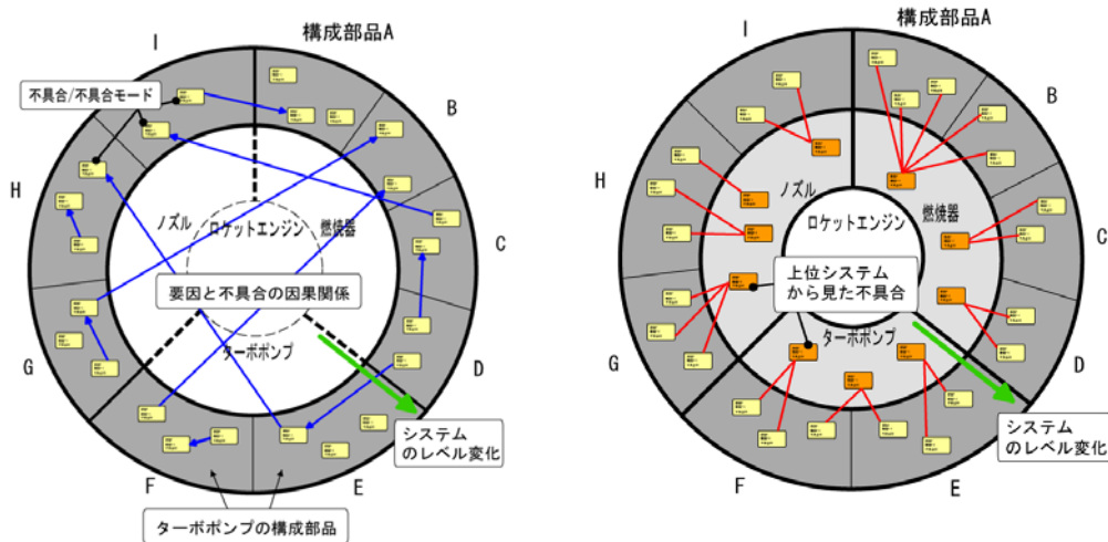
Figure 7. N2 chart view based on FMEA result.
