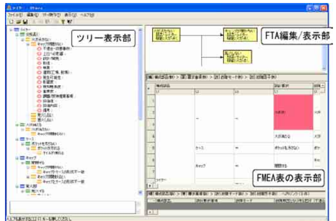
Figure 3. User interface of JAXA's detailed FMEA/FTA support tool.
