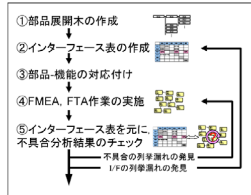
Figure 5. Interface N2 chart-based FMEA/FTA process.
