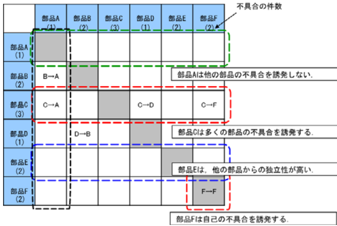
Figure 6. N2 chart view based on FMEA result.
