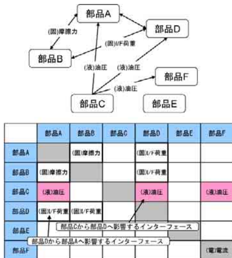
Figure 4. Description of interface as network and N2 chart.
